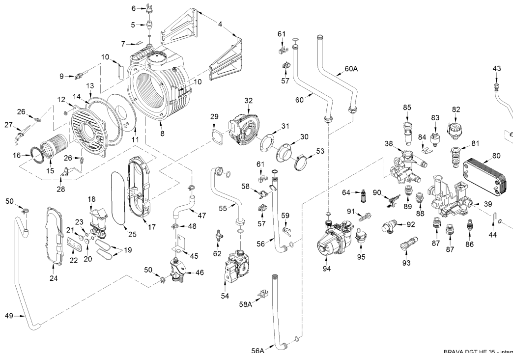
BRAVA DGT HE 35 - interno
